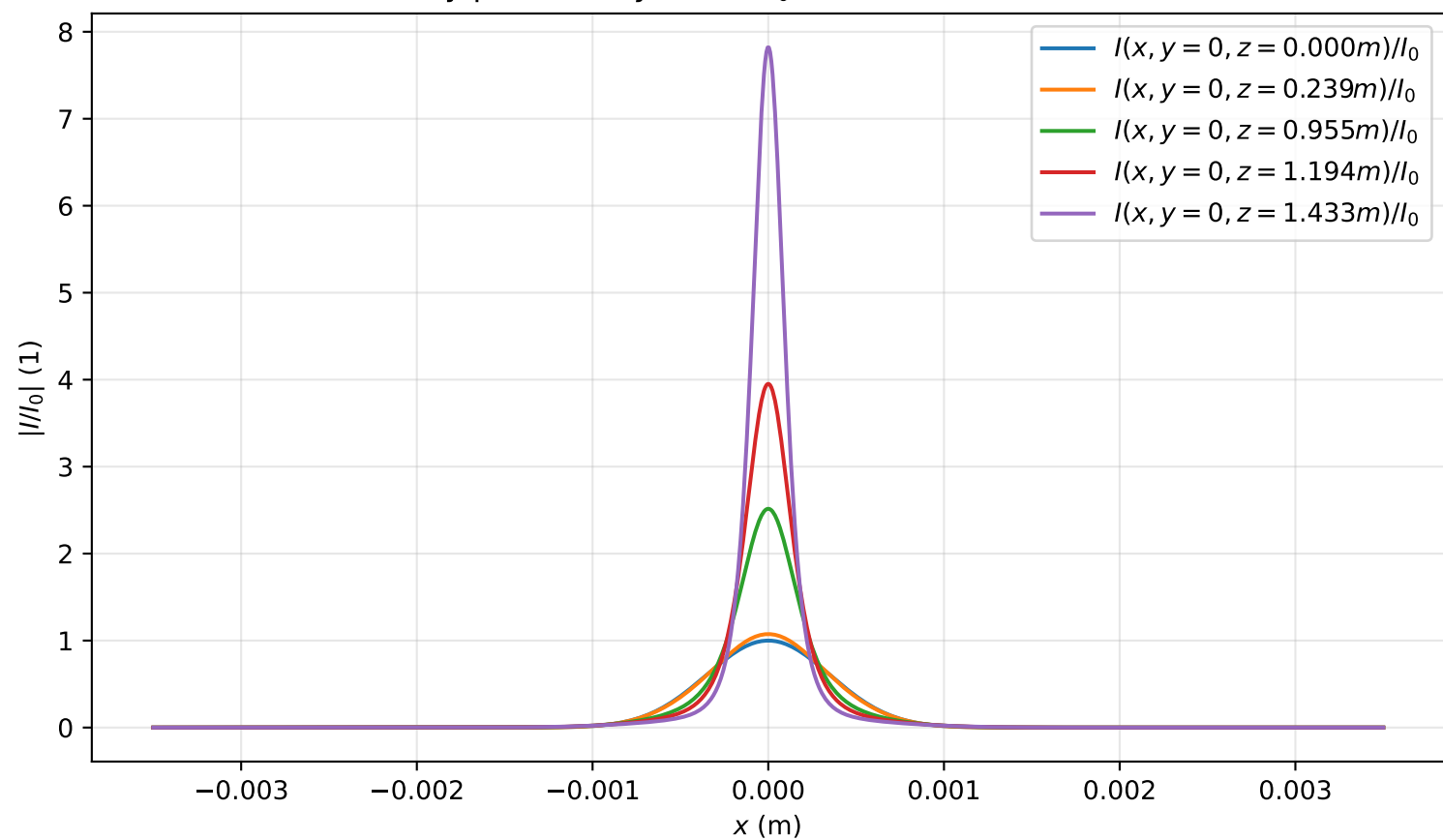
Intensity profile I(x, y = 0, z)/I_0 , P_{in}=1.5P_{cr} , artificial time
